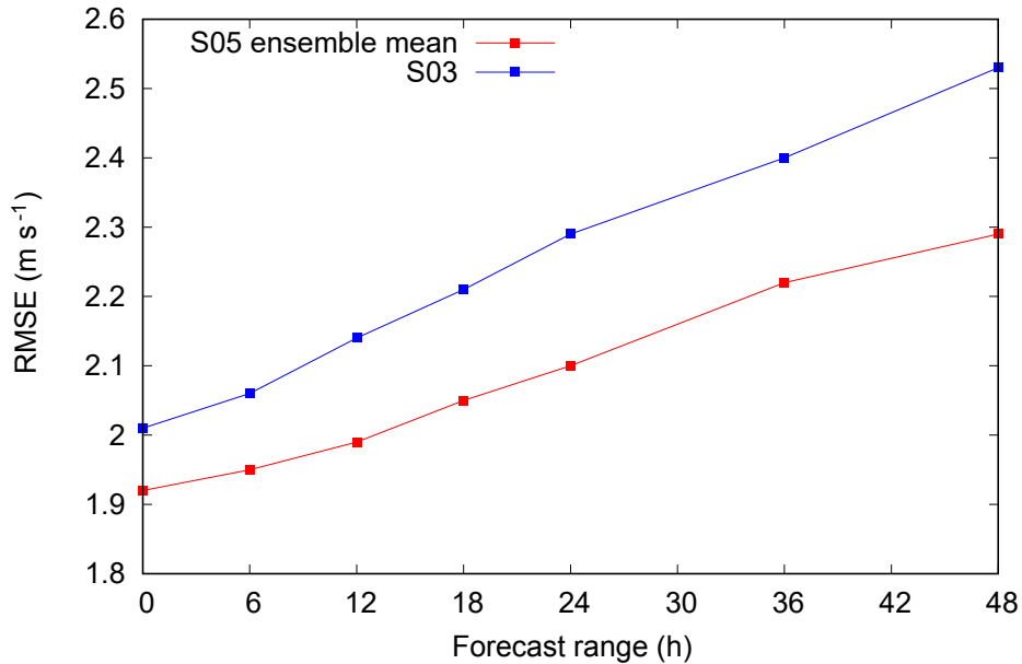
Wind speed forecast skill
