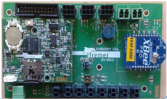
Micro-controller board with data storage and wireless link
