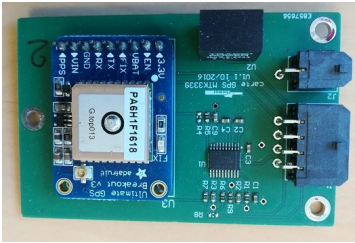
GPS board
